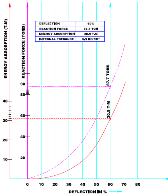
PERFORMANCE CURVE OF OUR "DIPTI" PNEUMATIC FENDER (SIZE: 2000 ØX 3500 MM LONG)
